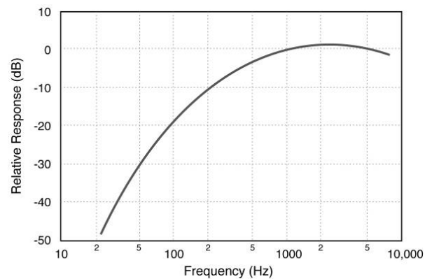
Figure 1 A-Weighting Frequency Response
